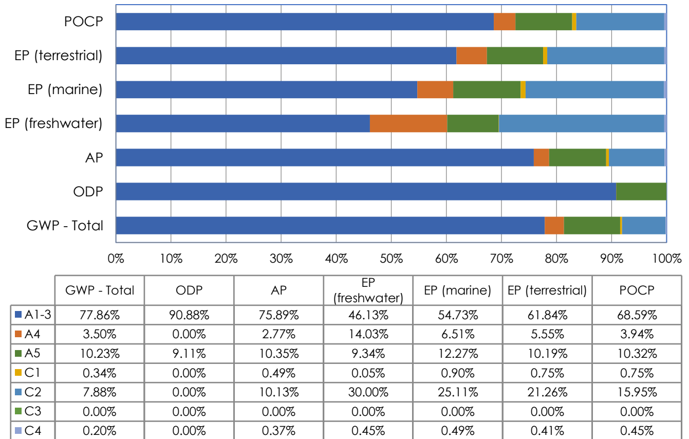
Figure 1 - shows the relative contribution of each life cycle stage to different environmental indicators for the carbon steel reinforcing bars manufactured by the secondary production route
